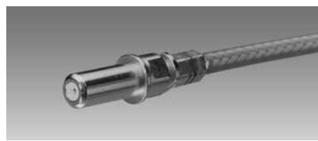
MIL-DTL-38999 LJT-R, JT-R, TV-R, SJT-R MS Type, Coax Size 8 Pin Assembled Contact
