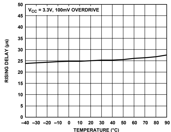
Figure 7. VIN1/VIN2/VIN3 to OUT1/OUT2/OUT3 Rising Delay vs. Temperature
