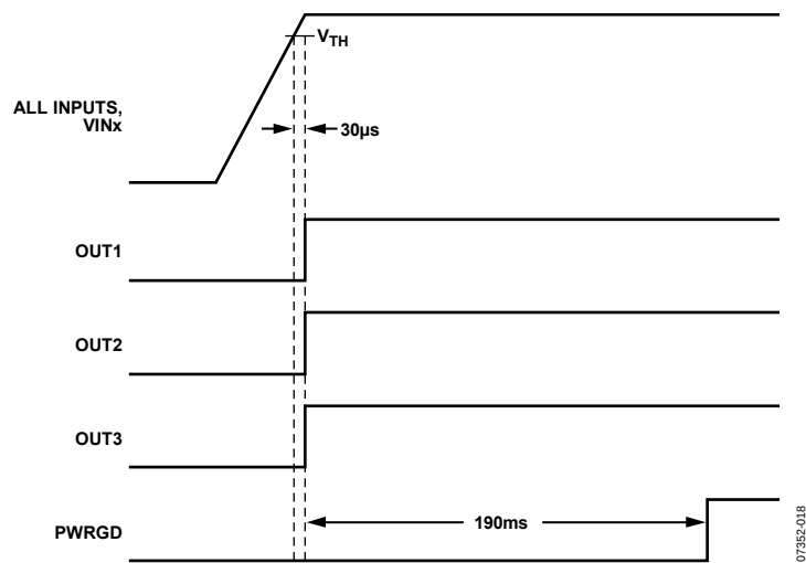
Figure 18. Power-Up Waveforms
