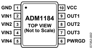
Figure 2. Pin Configuration
