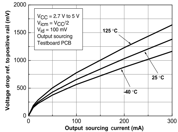
Figure 2. Voltage drop vs. output sourcing current
