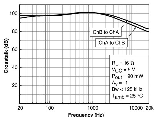
Figure 34. Crosstalk vs. frequency (R_L = 16\ \Omega, V_{CC} = 5\ \text{V}, P_{\text{out}} = 90\ \text{mW}, A_V = -1, BW < 125\ \text{kHz})
