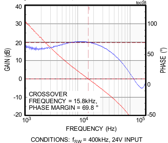
BODE PLOT (3.3V OUTPUT, 1A LOAD CURRENT)
