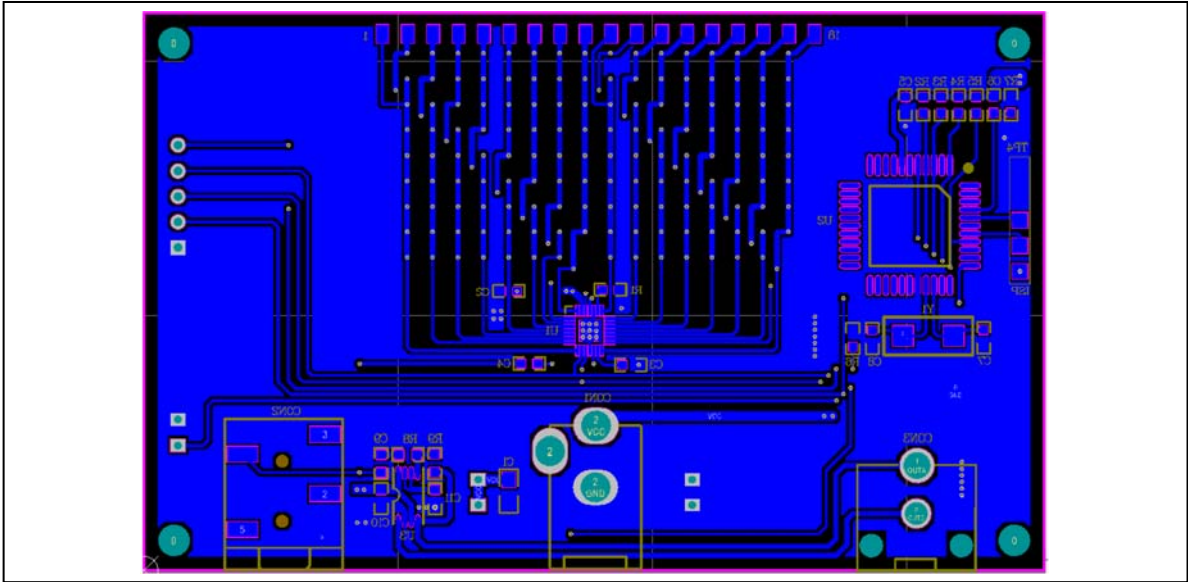
Figure 17: Board PCB Layout-Bottom Layer
