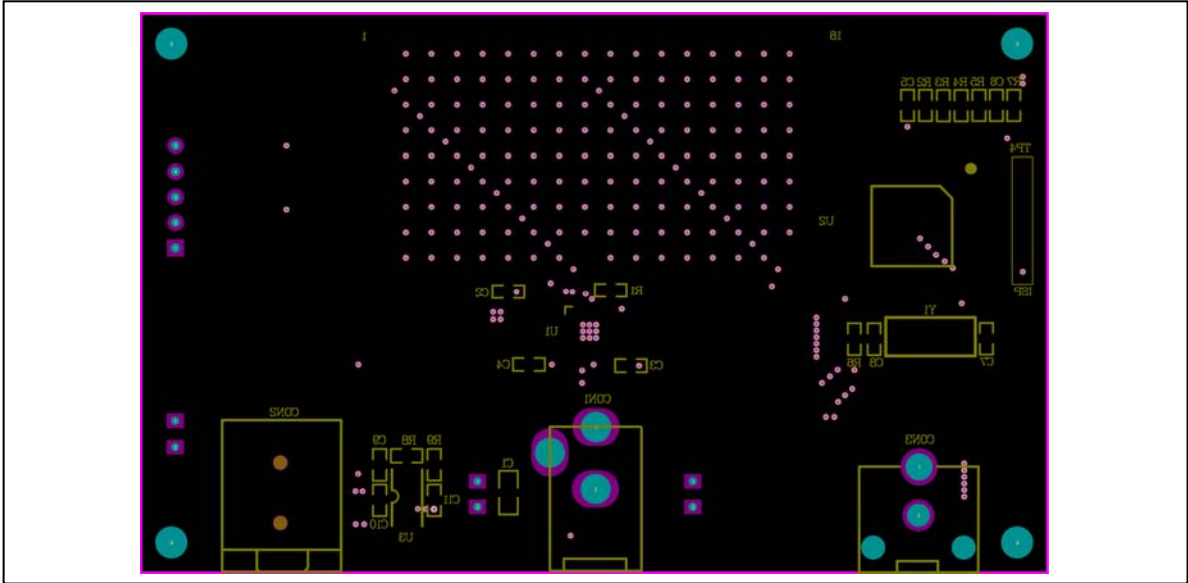
Figure 16: Board Component Placement Guide -Bottom Layer
