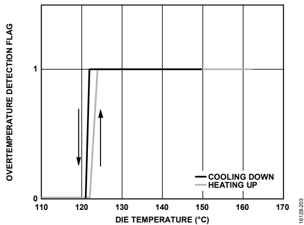
Figure 61. Overheat Warning
