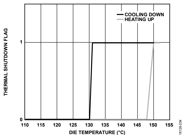
Figure 62. Overheat Shutdown
