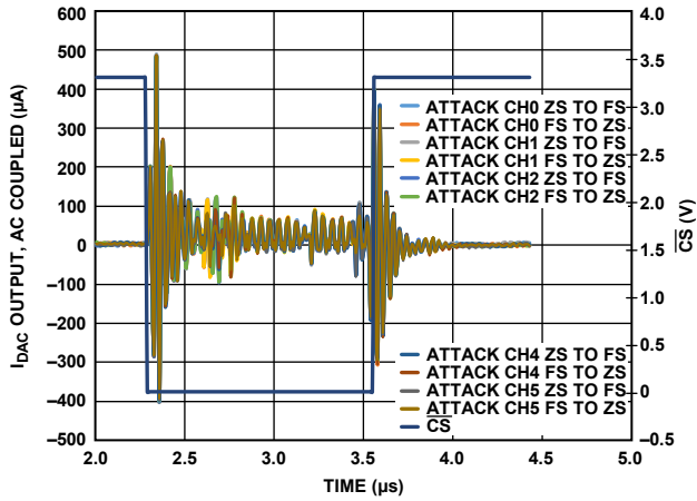
Figure 57. Digital Crosstalk
