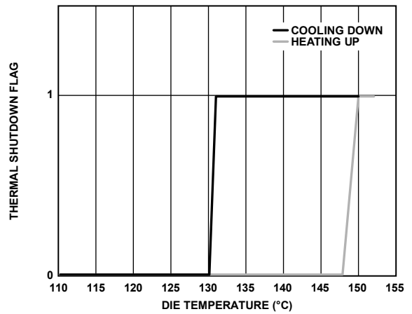
Figure 62. Overheat Shutdown
