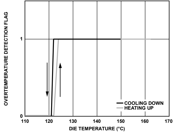
Figure 61. Overheat Warning
