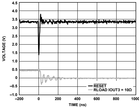
Figure 58. Reset Glitch
