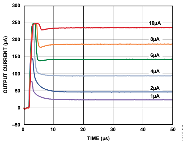
Figure 19. Power-Down Recovery, 1 µA to 10 µA
