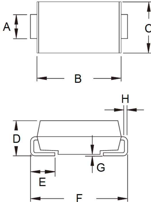
DO-214AA (SMB)
