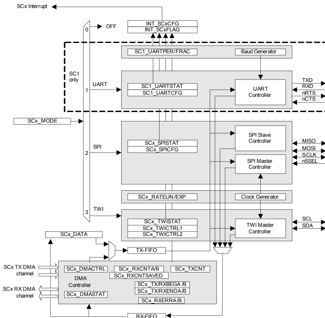
Figure 8.1. Serial Controller Block Diagram
