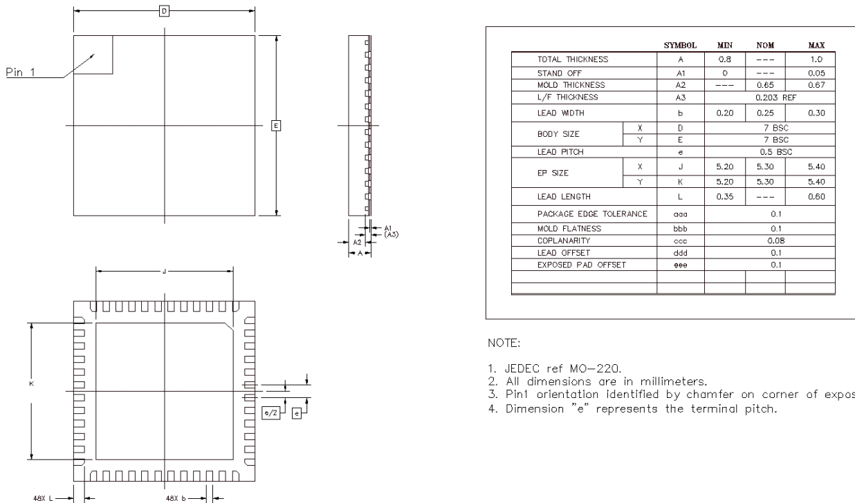
Figure 20.1. Package Drawing
