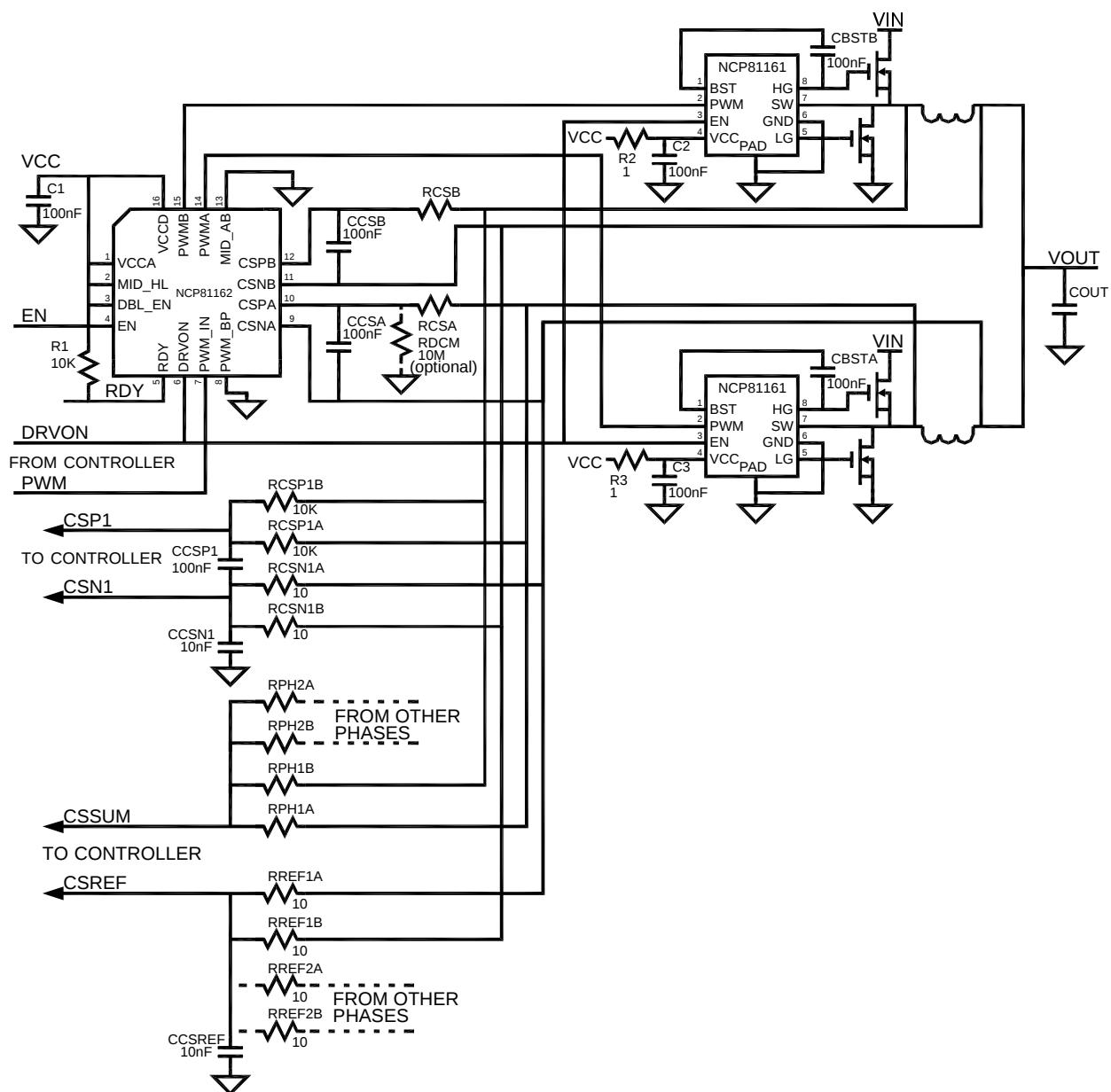
Figure 1. Application Schematic
