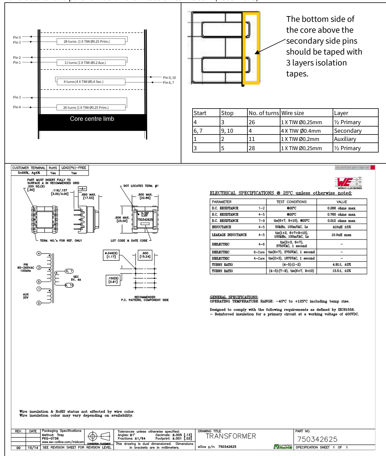
Figure 5 Transformer structure
