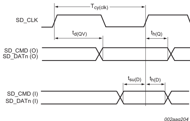
Fig 37. SD/MMC timing
