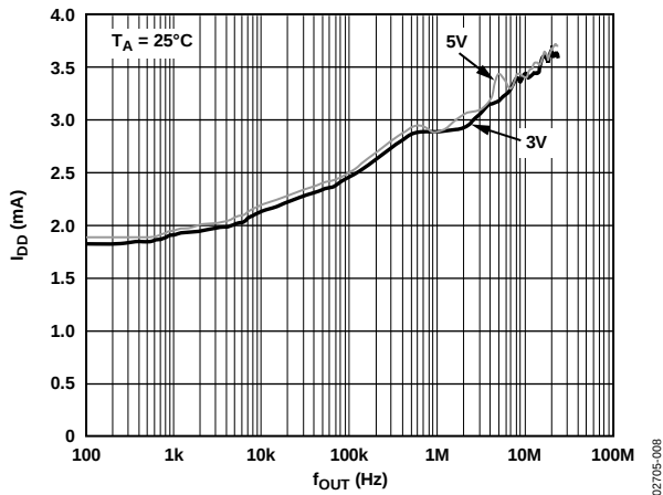
Figure 8. Typical I_{DD} vs. f_{OUT} for f_{MCLK} = 50\text{MHz}
