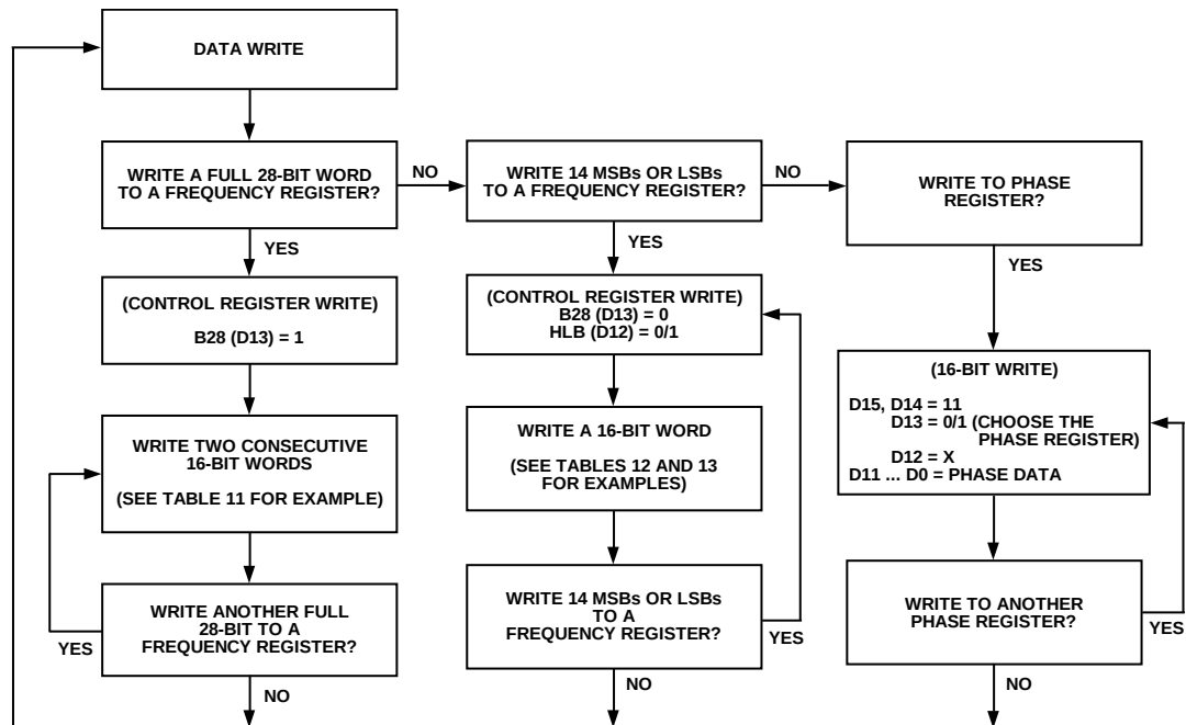
Figure 33. Data Write
