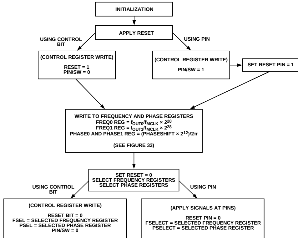
Figure 32. Initialization
