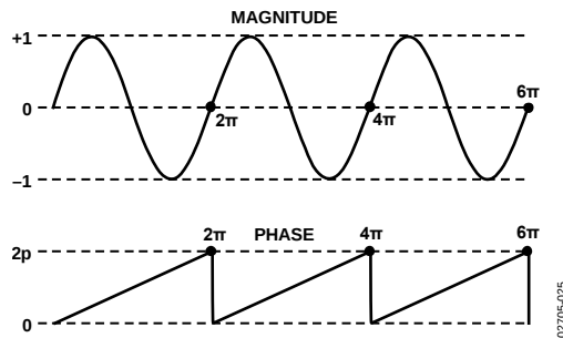
Figure 27. Sine Wave
