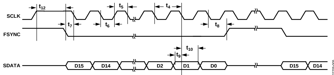
Figure 5. Serial Timing
