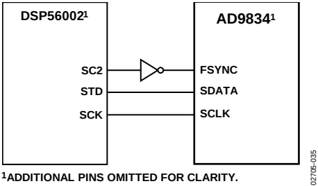
Figure 38. DSP56002 to AD9834 Interface
