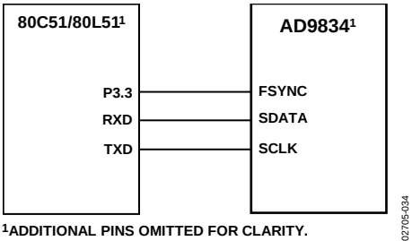
Figure 37. 80C51/80L51 to AD9834 Interface
