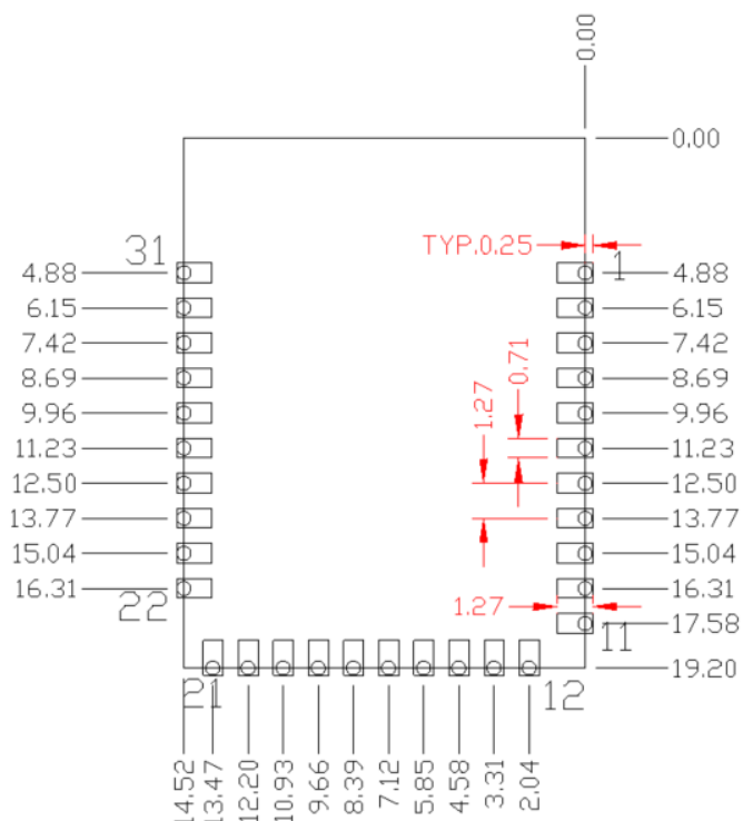
Top View (Seen on Host PCB)
