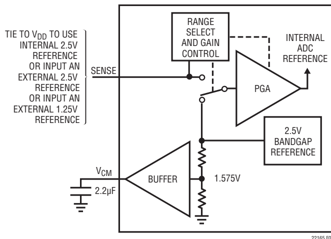
Figure 6. Reference Circuit
