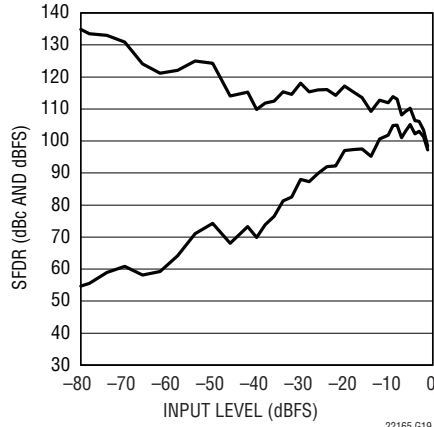
LTC2216 SFDR vs Input Level, f_{IN} = 70.5\text{MHz} , Dither "On"
