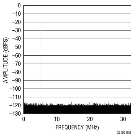
LTC2215 64k Point FFT, f_{IN} = 70.1\text{MHz} , -20dBFS, Dither "On"
