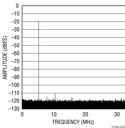
LTC2215 64k Point FFT, f_{IN} = 70.1\text{MHz} , -20dBFS, Dither "Off"
