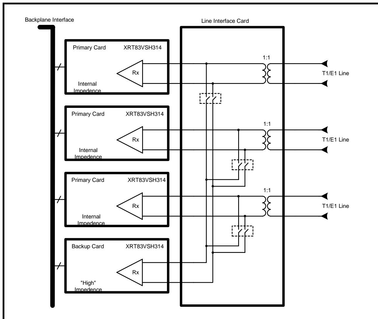
FIGURE 28. SIMPLIFIED BLOCK DIAGRAM OF THE RECEIVE INTERFACE FOR N+1 REDUNDANCY
