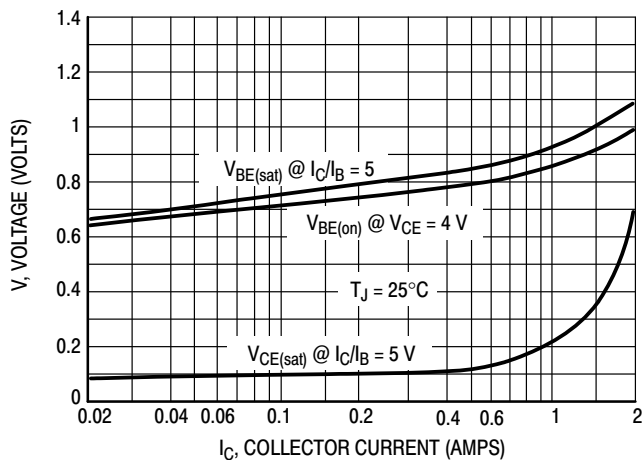
Figure 2. "On" Voltages
