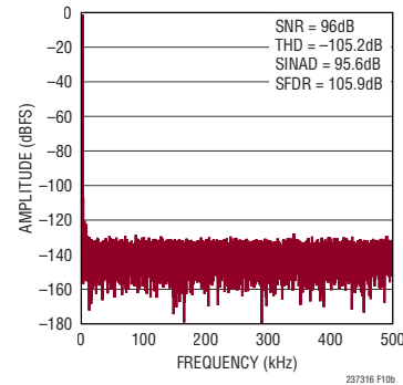
Figure 10b. 32k Point FFT f_{\text{SMPL}} = 1\text{MSPs} , f_{\text{IN}} = 1\text{kHz} for Circuit Shown in Figure 10a
