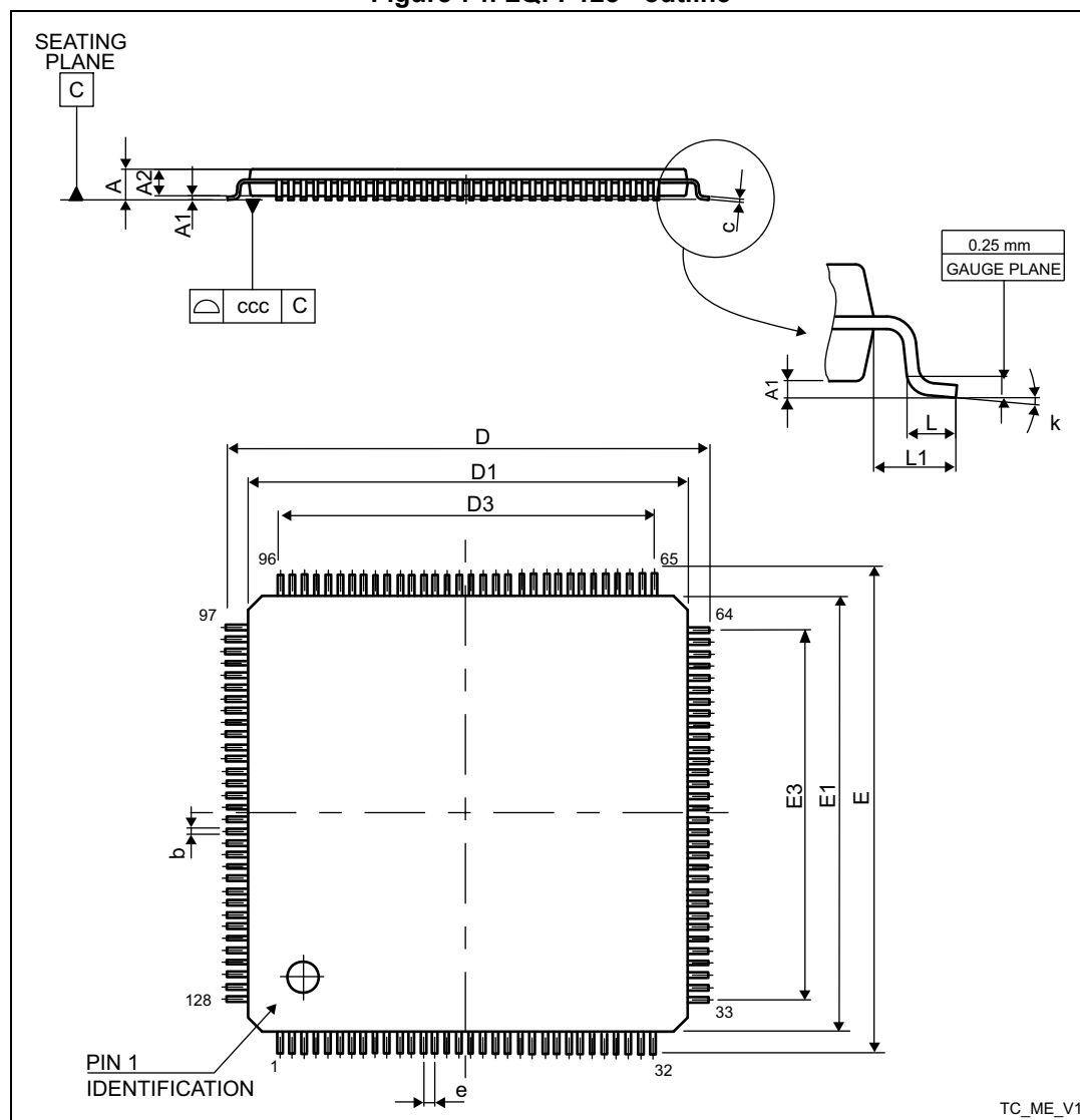
Figure 74. LQFP128 - outline
