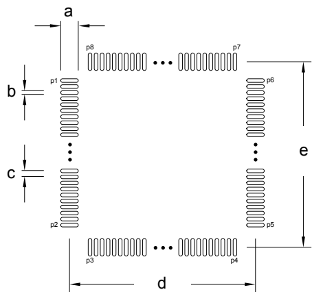
Figure 8.2. LQFP100 PCB Land Pattern
