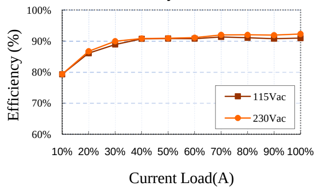
CBM100S360 Efficiency VS . Load
