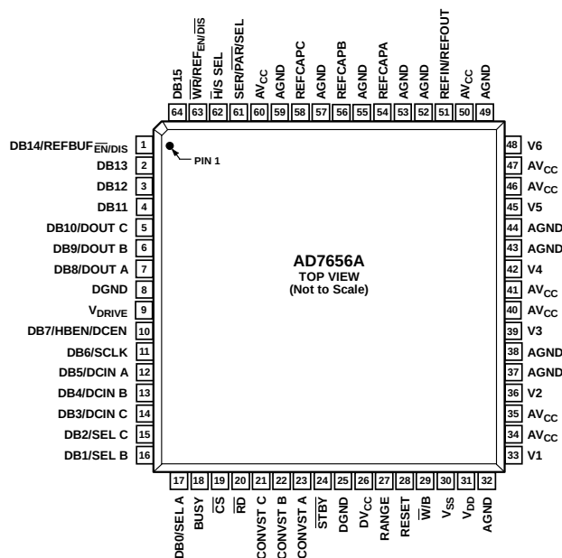
Figure 3. Pin Configuration
