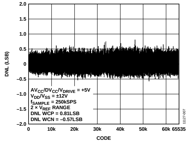
Figure 7. Typical DNL
