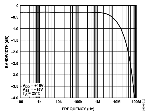
Figure 26. ADGS1408 Insertion Loss vs. Frequency, ±15 V Dual Supply
