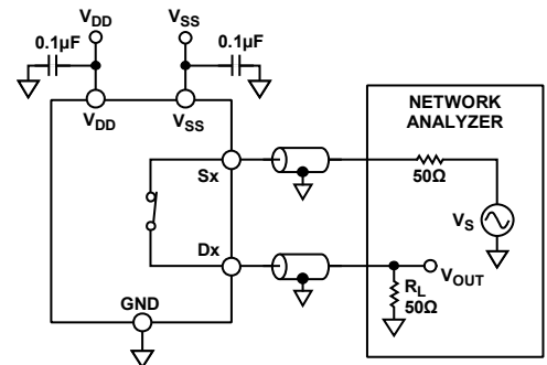
Figure 37. -3 dB Bandwidth
