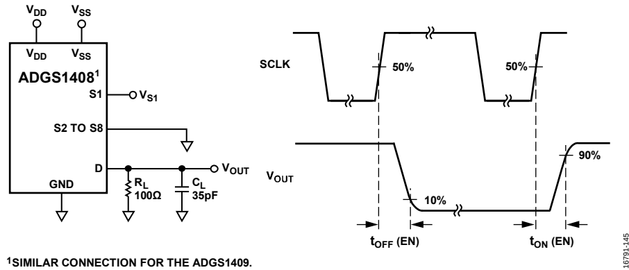
Figure 41. Switching Times, t_{\text{ON}}(\text{EN}) and t_{\text{OFF}}(\text{EN})
