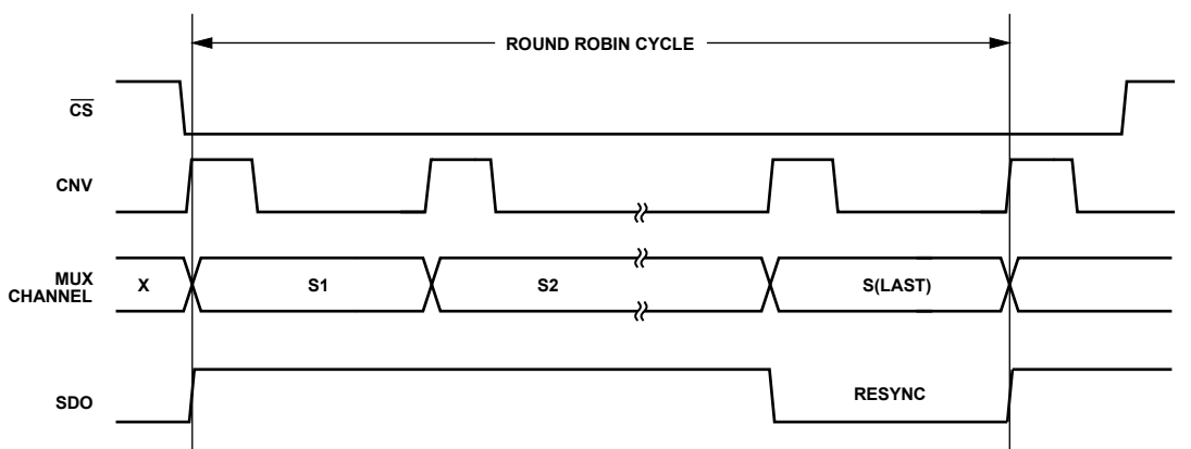
Figure 51. Round Robin Mode Interface Example
