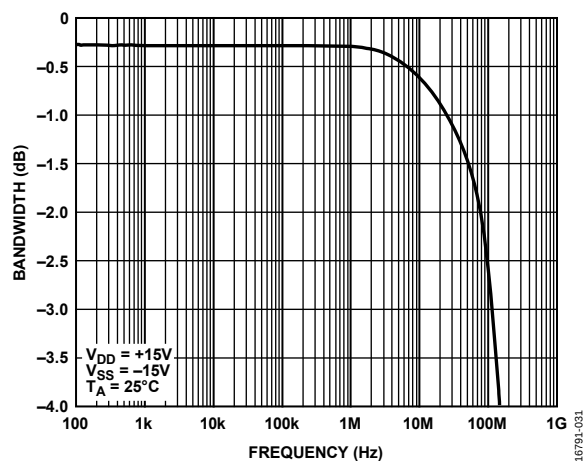
Figure 27. ADGS1409 Insertion Loss vs. Frequency, \pm 15 V Dual Supply
