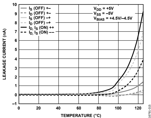
Figure 17. Leakage Current vs. Temperature, \pm 5 V Dual Supply
