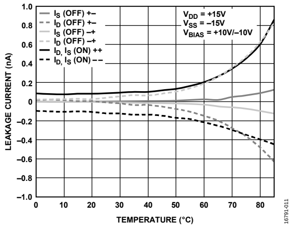
Figure 15. Leakage Current vs. Temperature, \pm 15 V Dual Supply
