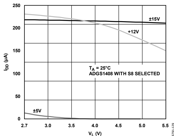
Figure 29. I_{DD} vs. V_L
