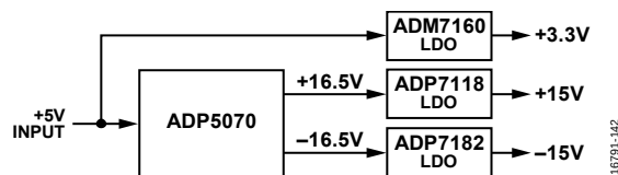
Figure 54. Bipolar Power Solution
