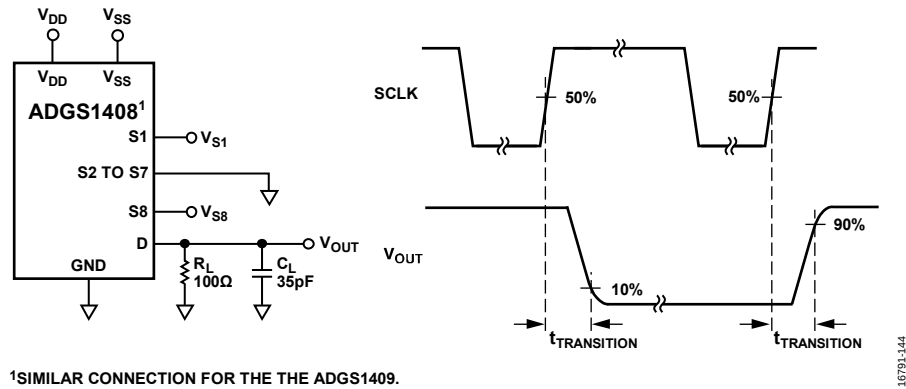
Figure 40. Transition Time, t_{\text{TRANSITION}}
