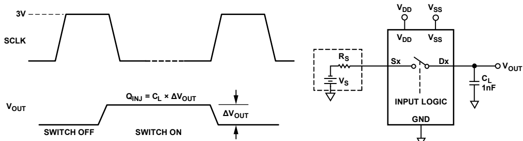
Figure 42. Charge Injection, Q_{\text{INJ}}
