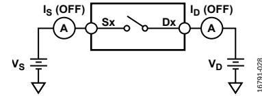
Figure 35. Off Leakage
