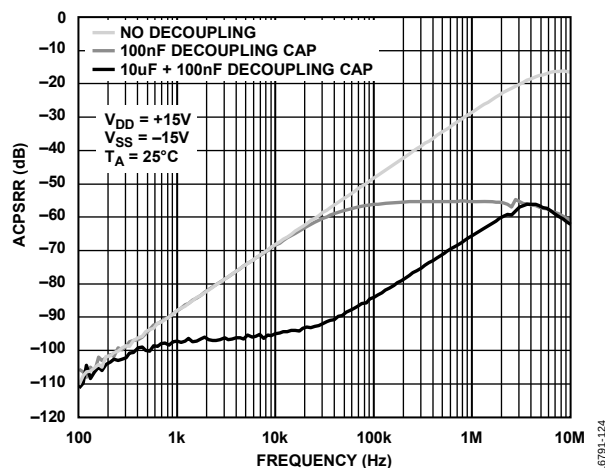
Figure 24. AC Power Supply Rejection Ratio (ACPSRR) vs. Frequency, ±15 V Dual Supply
