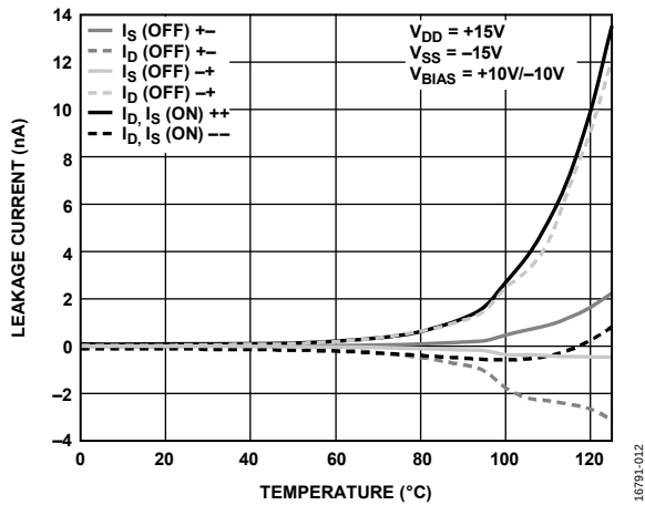
Figure 16. Leakage Current vs. Temperature, \pm 15 V Dual Supply
