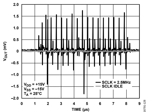
Figure 28. Digital Feedthrough
