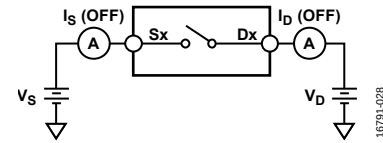
Figure 35. Off Leakage
