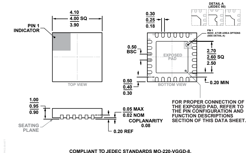
Figure 55. 24-Lead Lead Frame Chip Scale Package [LFCSP] 4 mm × 4 mm Body and 0.95 mm Package Height (CP-24-17)
