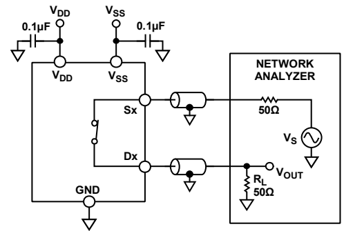
Figure 37. -3 dB Bandwidth
