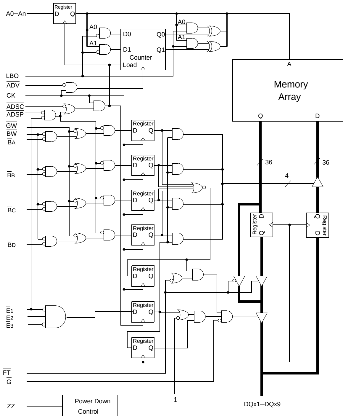
GS816118/32/36D Block Diagram
