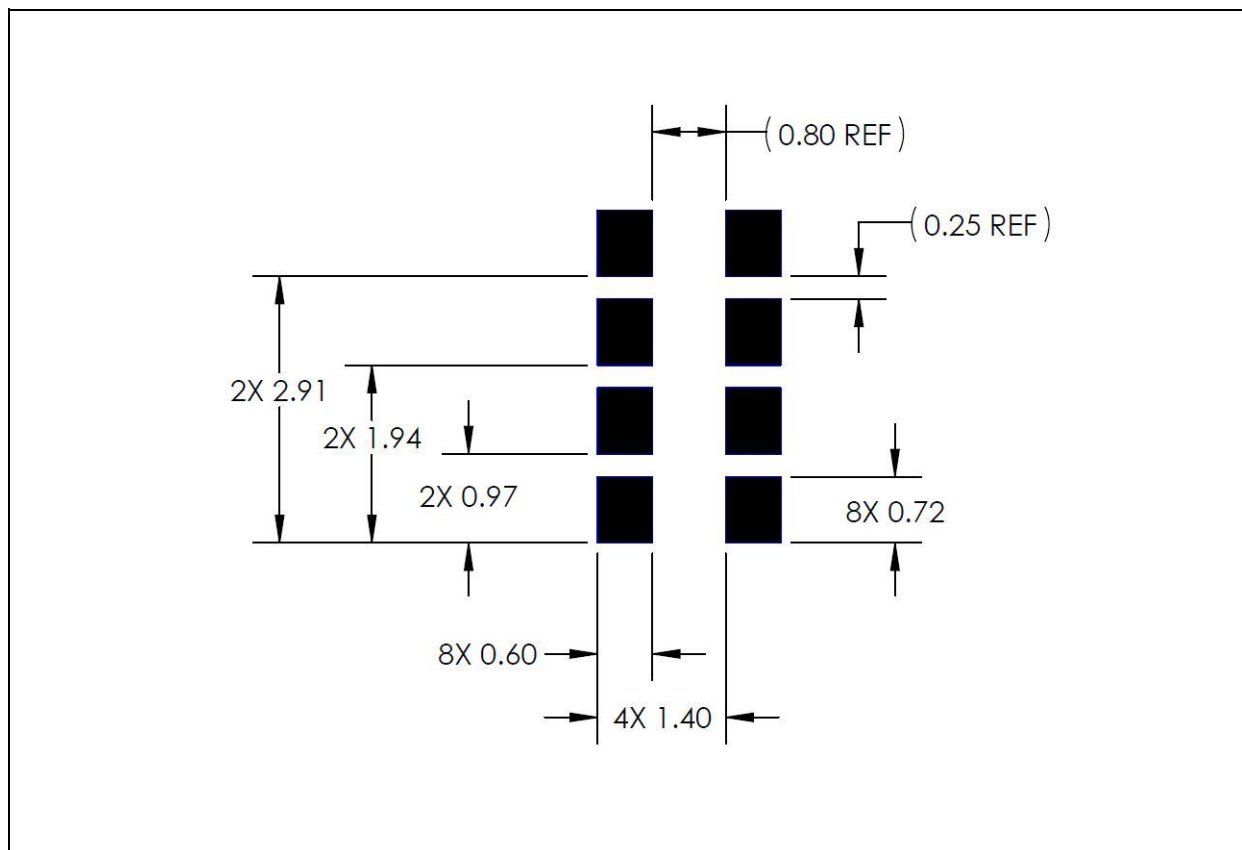
Figure 51: Suggested Module PCB Layout
