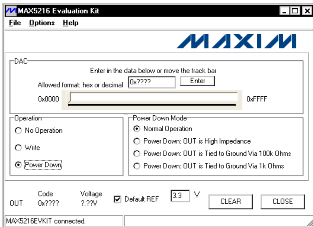
Figure 3. MAX5216 EV Kit Software Main Window (Power-Down Mode)
