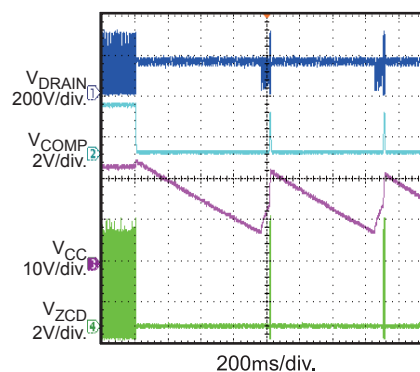
Over Voltage Protection LED Load Open When Working
