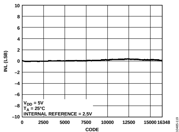
Figure 16. AD5685R INL
