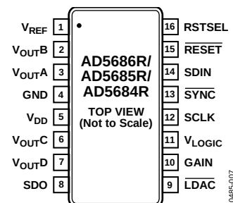
Figure 7. 16-Lead TSSOP Pin Configuration
