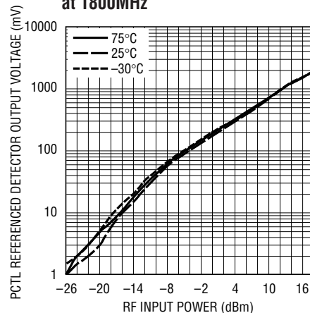
LTC4400-2 Detector Characteristics at 1800MHz
