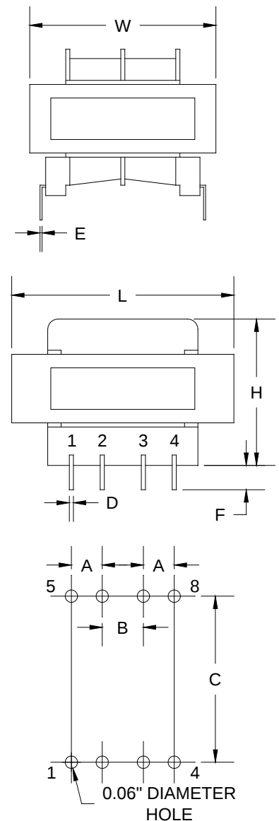
Board Layout
