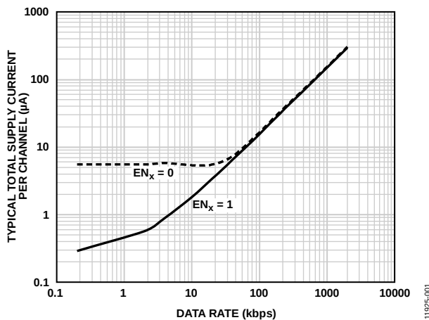
Figure 3. Typical Total Supply Current (IDD1 + IDD2) per Channel (VDDx = 3.3 V) as a Function of Data Rate
