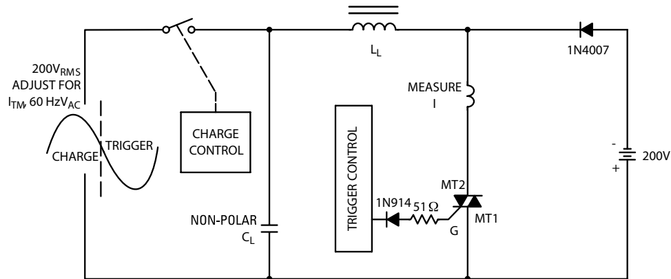
Figure 8. Simplified Test Circuit to Measure the Critical Rate of Rise of Commutating Current ( di/dt )
