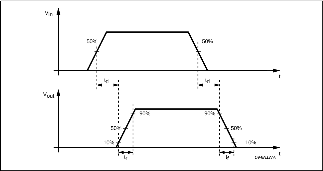
Figure 5. Switching waveforms
