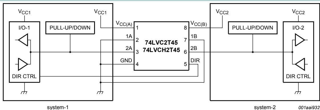
Pull-up or pull-down only needed for 74LVC2T45.
