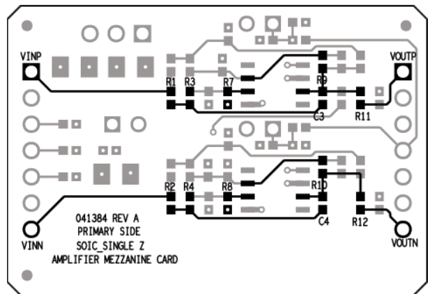
Figure 11. Sallen-Key, High-Pass Filter for 8-Lead SOIC, Single Board Connections
