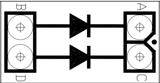
SCHEMATIC DIAGRAM 591833-2
