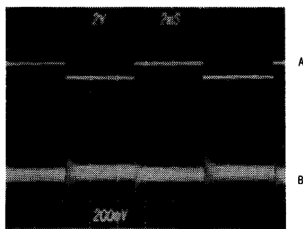
A: V_{IN} , 2V/div, 3V TO 4V B: V_{OUT} , 200mV/div, AC-COUPLED I_{OUT} = 180\text{mA}
