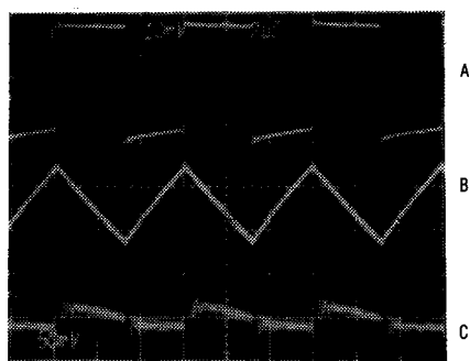
A: SWITCH VOLTAGE (LX PIN), 2V/div B: INDUCTOR CURRENT, 200mA/div C: OUTPUT VOLTAGE RIPPLE, 50mV/div V_{IN} = 3\text{V} , I_{OUT} = 150\text{mA}
