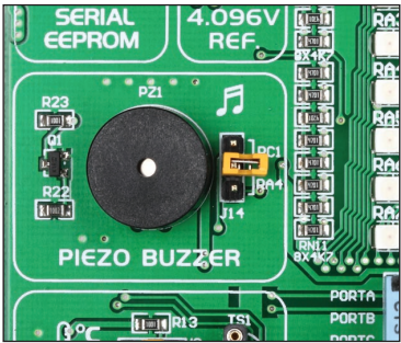
Figure 9-1: Piezo buzzer
