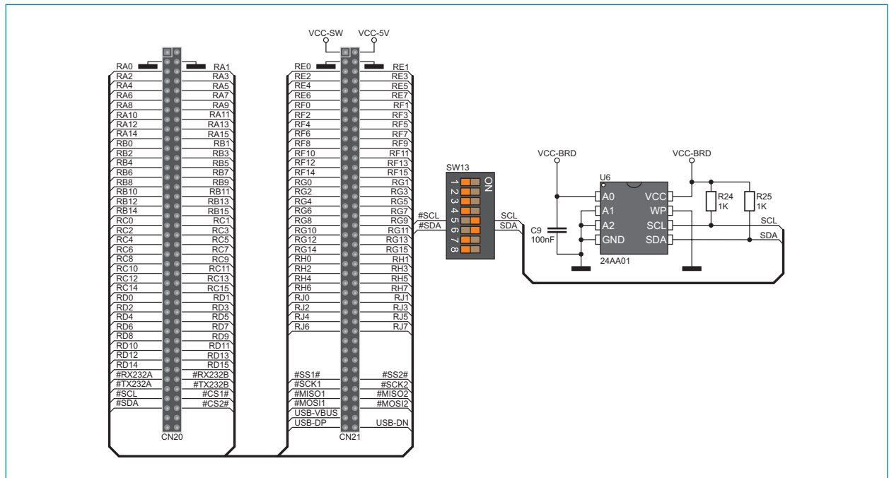
Figure 8-2: EEPROM module connection schematic
