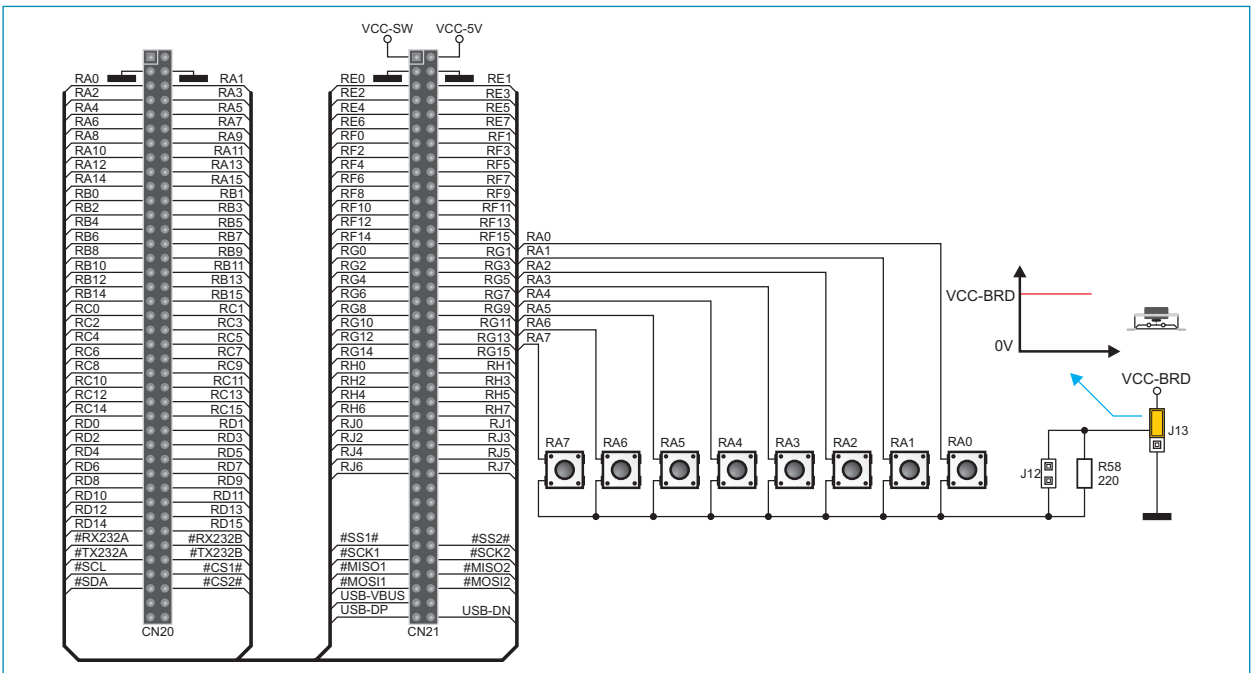
Figure 13-2: Push buttons and port PORT0 connection schematic
