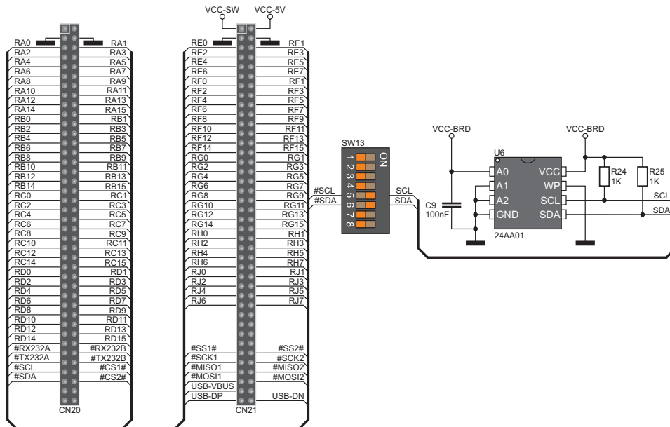
Figure 8-2: EEPROM module connection schematic
