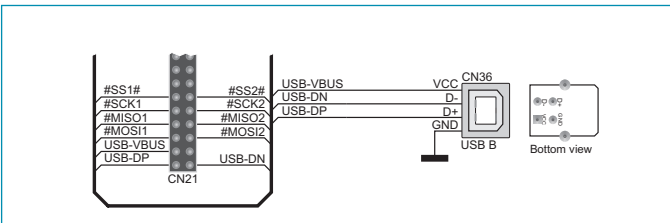
Figure 7-2: USB connector connection schematic
