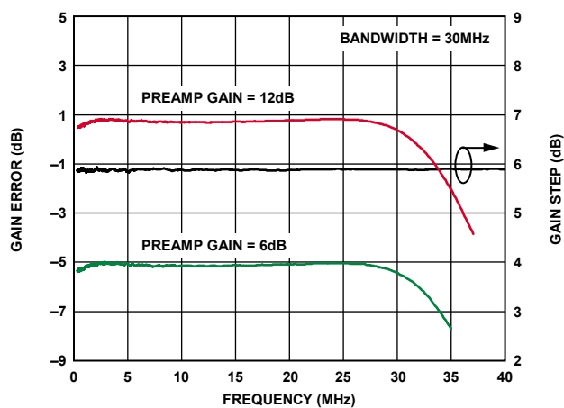
Figure 9. 6 dB Gain Step and Gain Error vs. Frequency (Bandwidth Setting = 30 MHz, V_{\text{GAIN}} = 0\ \text{V} )
