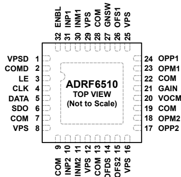
Figure 4. Pin Configuration
