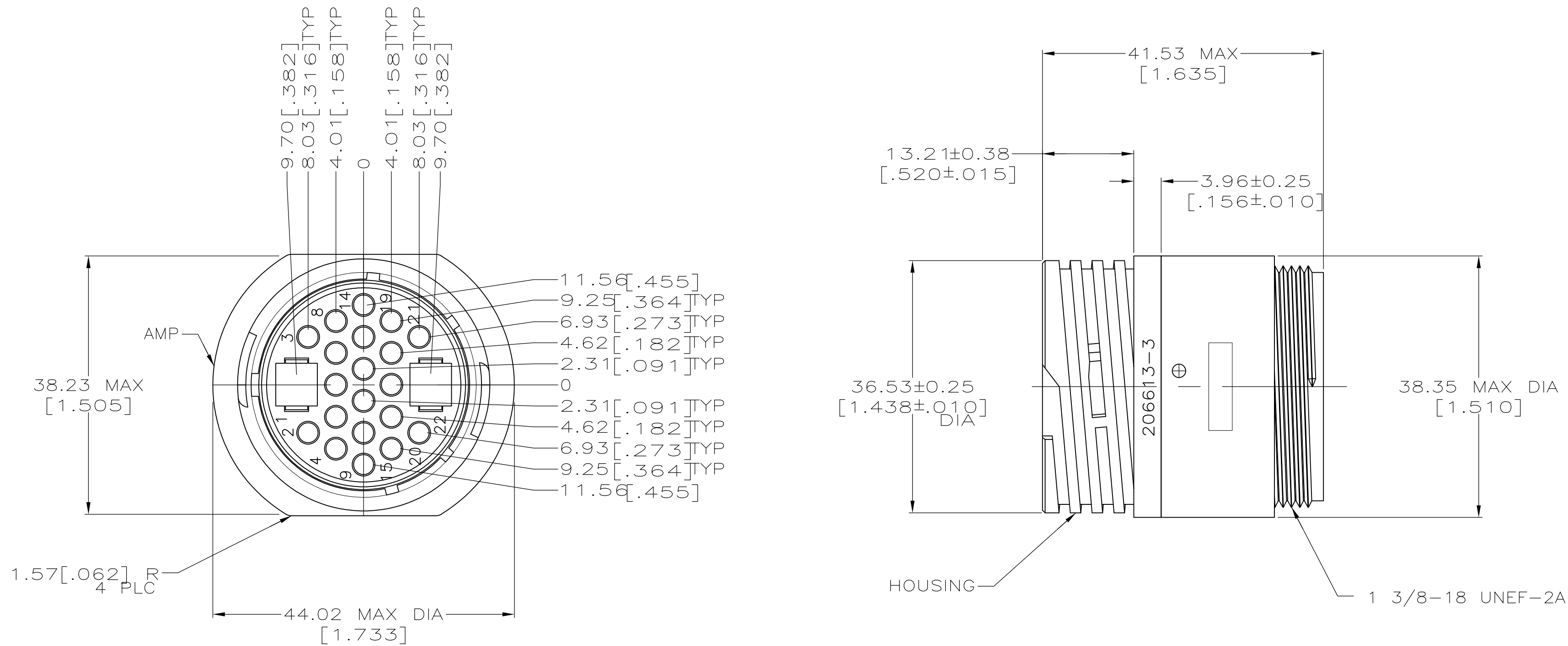
DETAIL B
