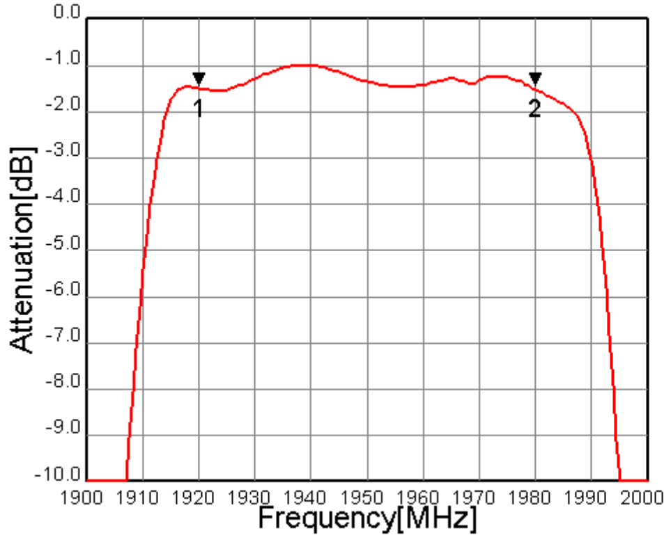
Fig.3 In-band Characteristics
