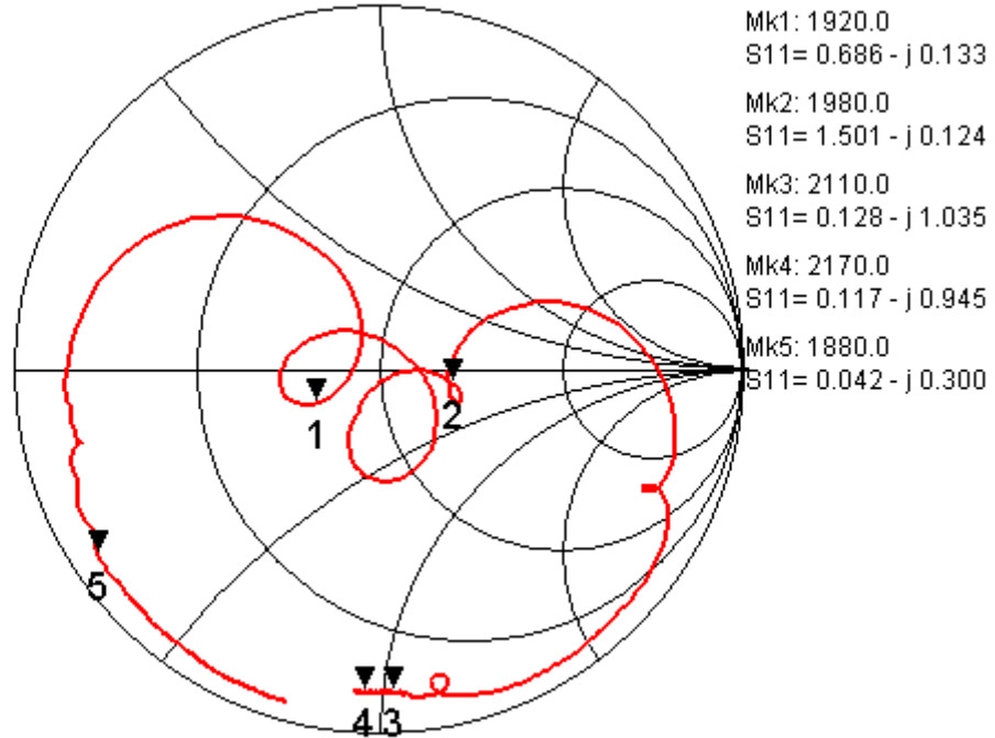
Fig.5 Impedance (S11)
