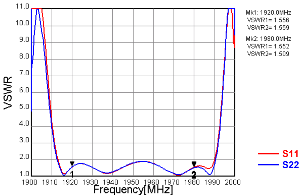
Fig.2 VSWR
