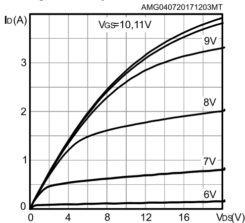
Figure 8: Output characteristics
