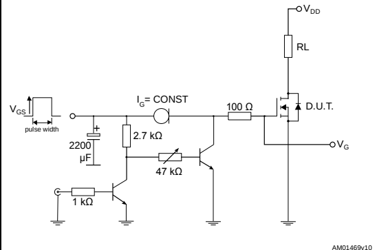
Figure 19: Test circuit for gate charge behavior
