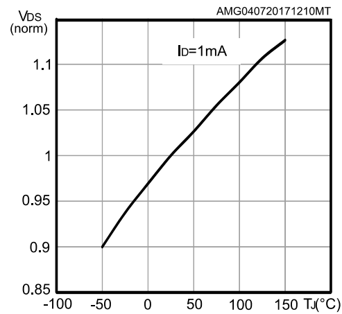
Figure 16: Normalized VDS vs temperature
