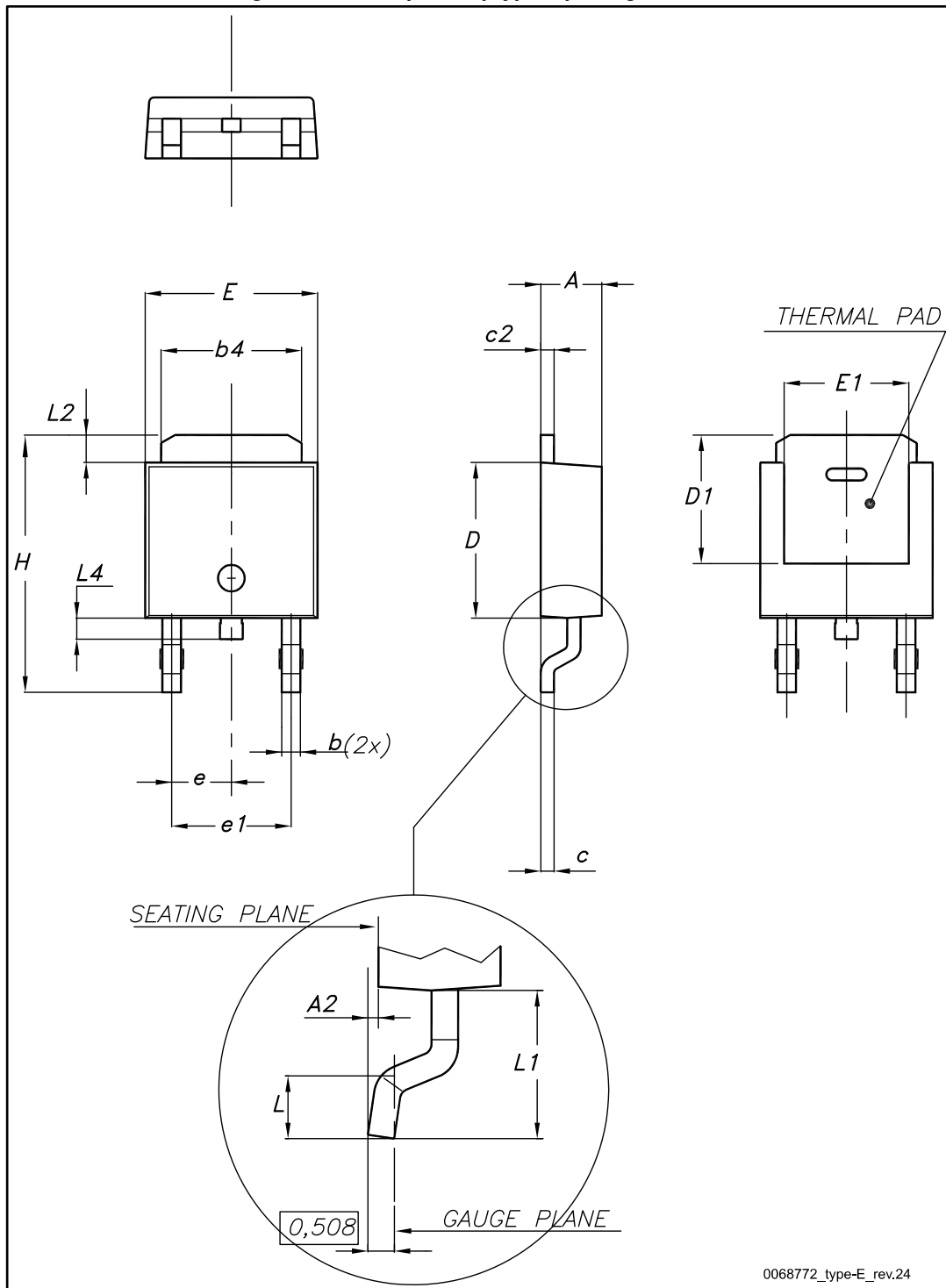
Figure 26: DPAK (TO-252) type E package outline
