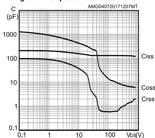
Figure 12: Capacitance variations
